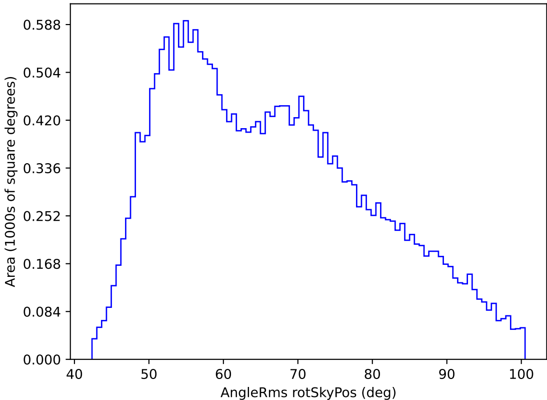
ddf_loaded_fl1_v3.4_10yrs All sky g band: AngleRms rotSkyPos
