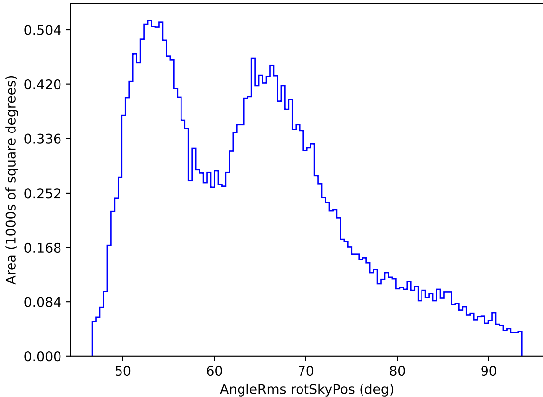
ddf_loaded_fl1_v3.4_10yrs All sky all bands: AngleRms rotSkyPos
