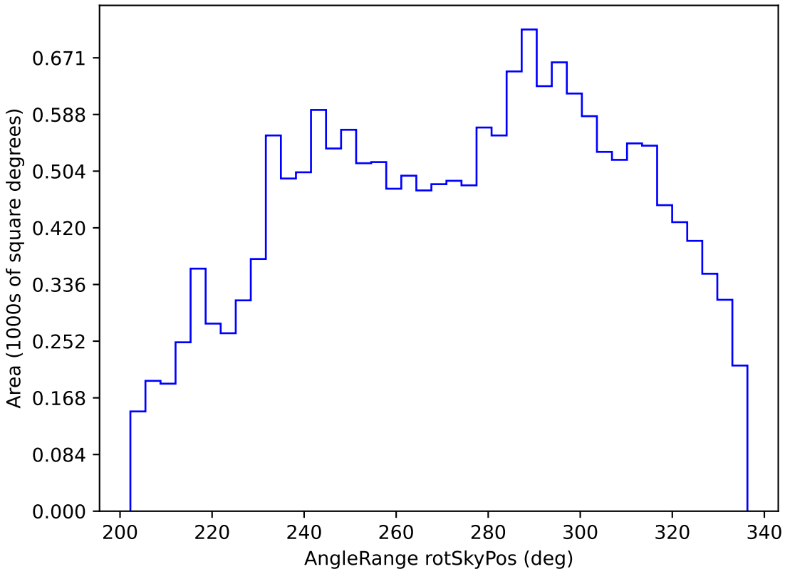
ddf_loaded_fl1_v3.4_10yrs WFD y band: AngleRange rotSkyPos
