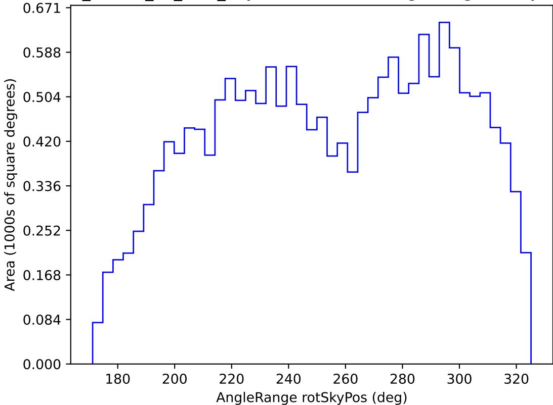
ddf_loaded_fl1_v3.4_10yrs WFD u band: AngleRange rotSkyPos
