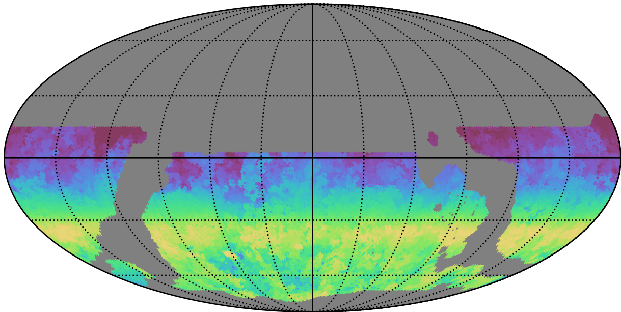
ddf_loaded_fl1_v3.4_10yrs WFD r band: AngleRange rotSkyPos
