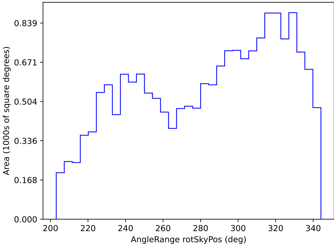
ddf_loaded_fl1_v3.4_10yrs WFD r band: AngleRange rotSkyPos
