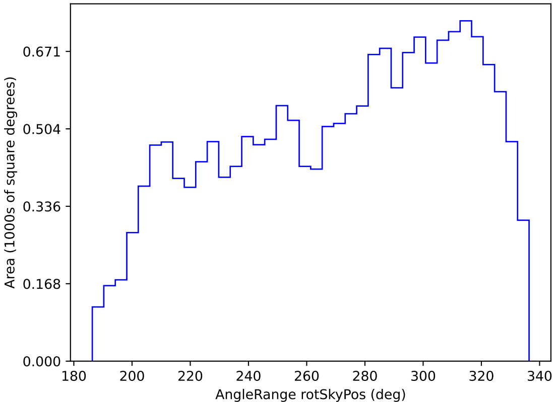
ddf_loaded_fl1_v3.4_10yrs WFD g band: AngleRange rotSkyPos
