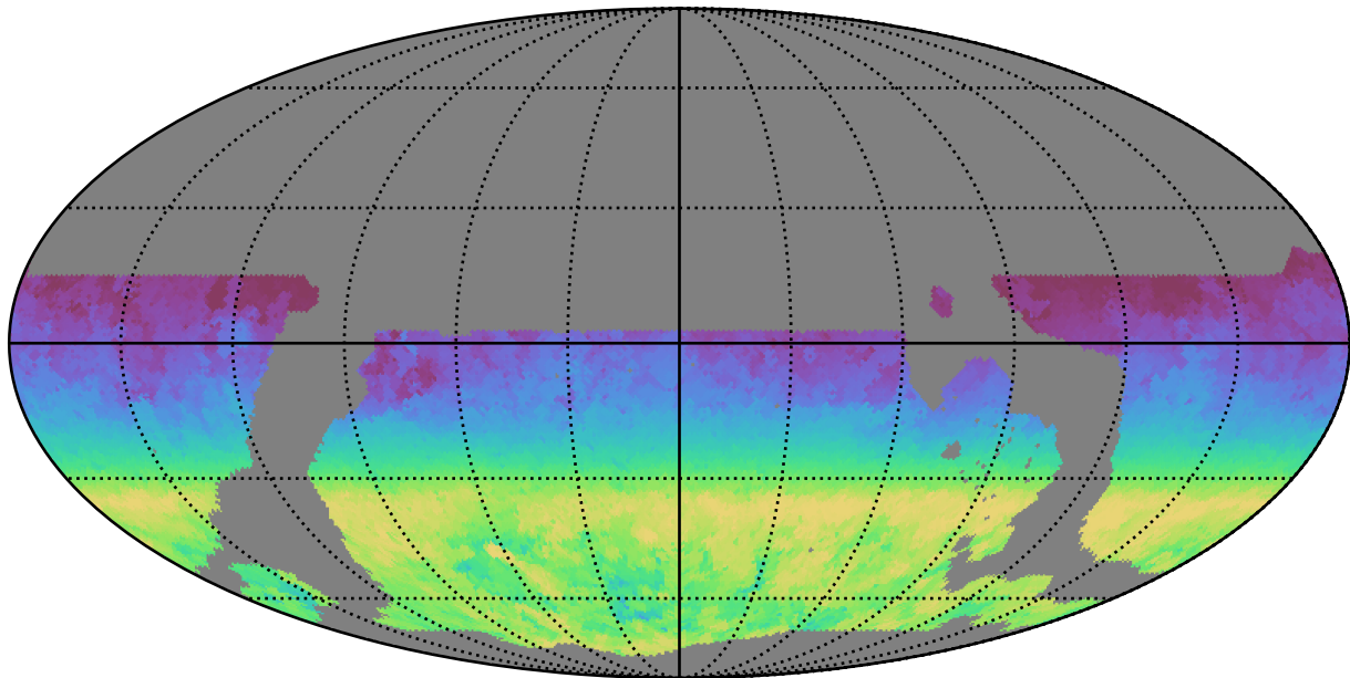
ddf_loaded_fl1_v3.4_10yrs WFD all bands: AngleRange rotSkyPos
