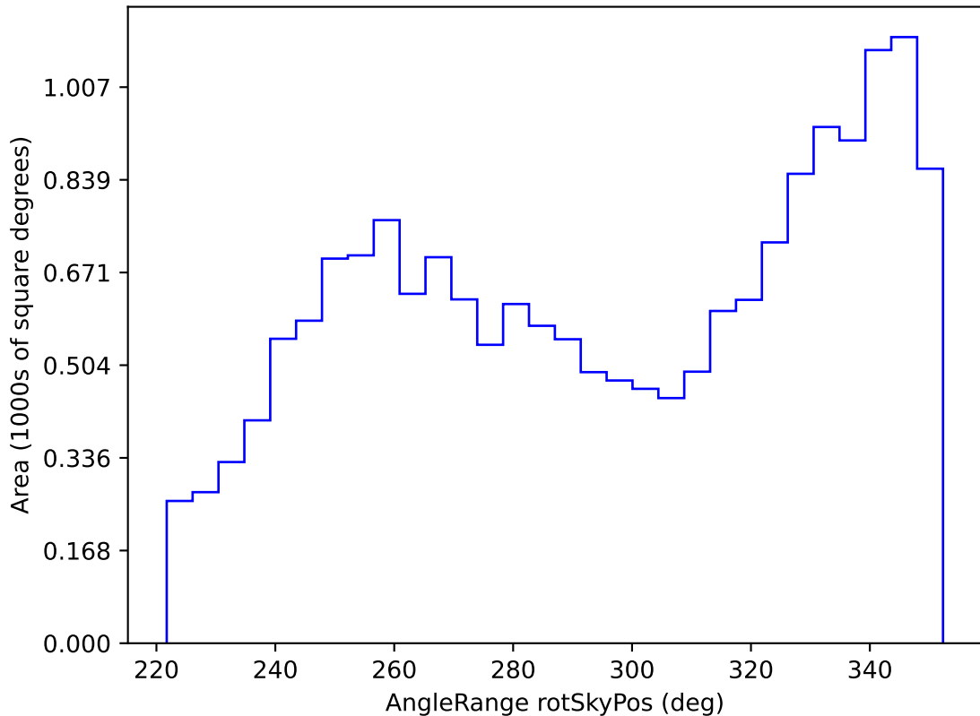
ddf_loaded_fl1_v3.4_10yrs WFD all bands: AngleRange rotSkyPos
