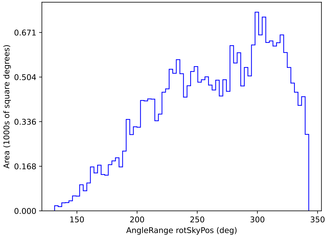
ddf_loaded_fl1_v3.4_10yrs All sky z band: AngleRange rotSkyPos
