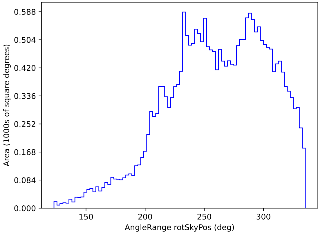
ddf_loaded_fl1_v3.4_10yrs All sky y band: AngleRange rotSkyPos
