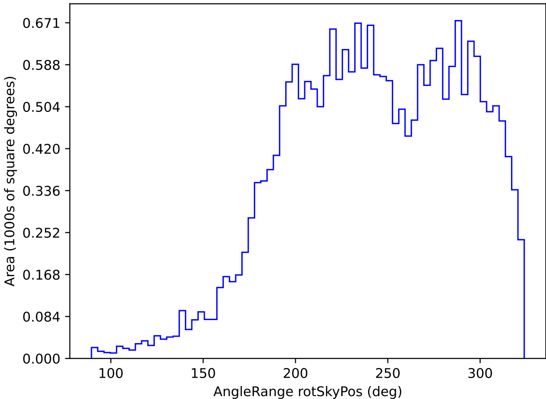
ddf_loaded_fl1_v3.4_10yrs All sky u band: AngleRange rotSkyPos
