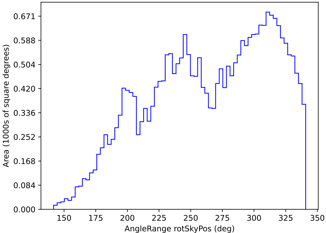
ddf_loaded_fl1_v3.4_10yrs All sky i band: AngleRange rotSkyPos
