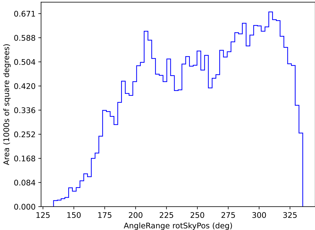
ddf_loaded_fl1_v3.4_10yrs All sky g band: AngleRange rotSkyPos
