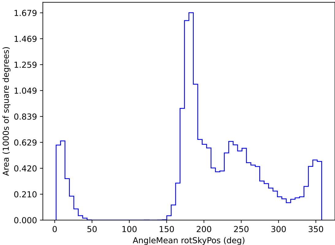
ddf_loaded_fl1_v3.4_10yrs WFD z band: AngleMean rotSkyPos
