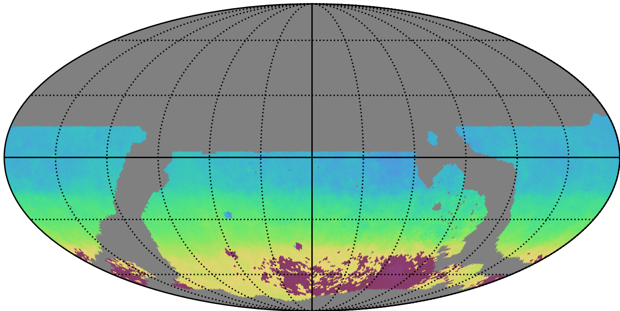
ddf_loaded_fl1_v3.4_10yrs WFD y band: AngleMean rotSkyPos
