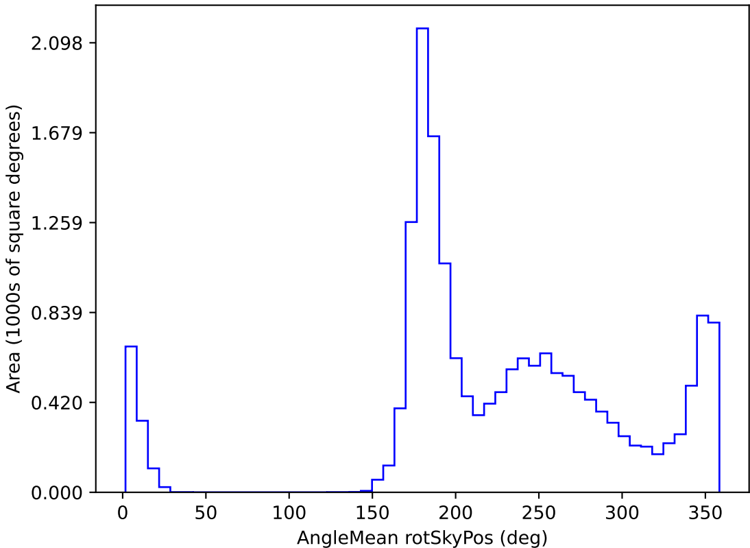
ddf_loaded_fl1_v3.4_10yrs WFD y band: AngleMean rotSkyPos
