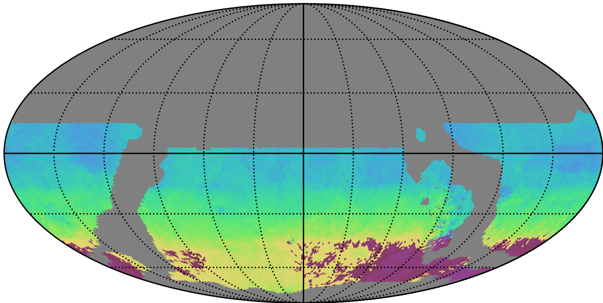
ddf_loaded_fl1_v3.4_10yrs WFD u band: AngleMean rotSkyPos
