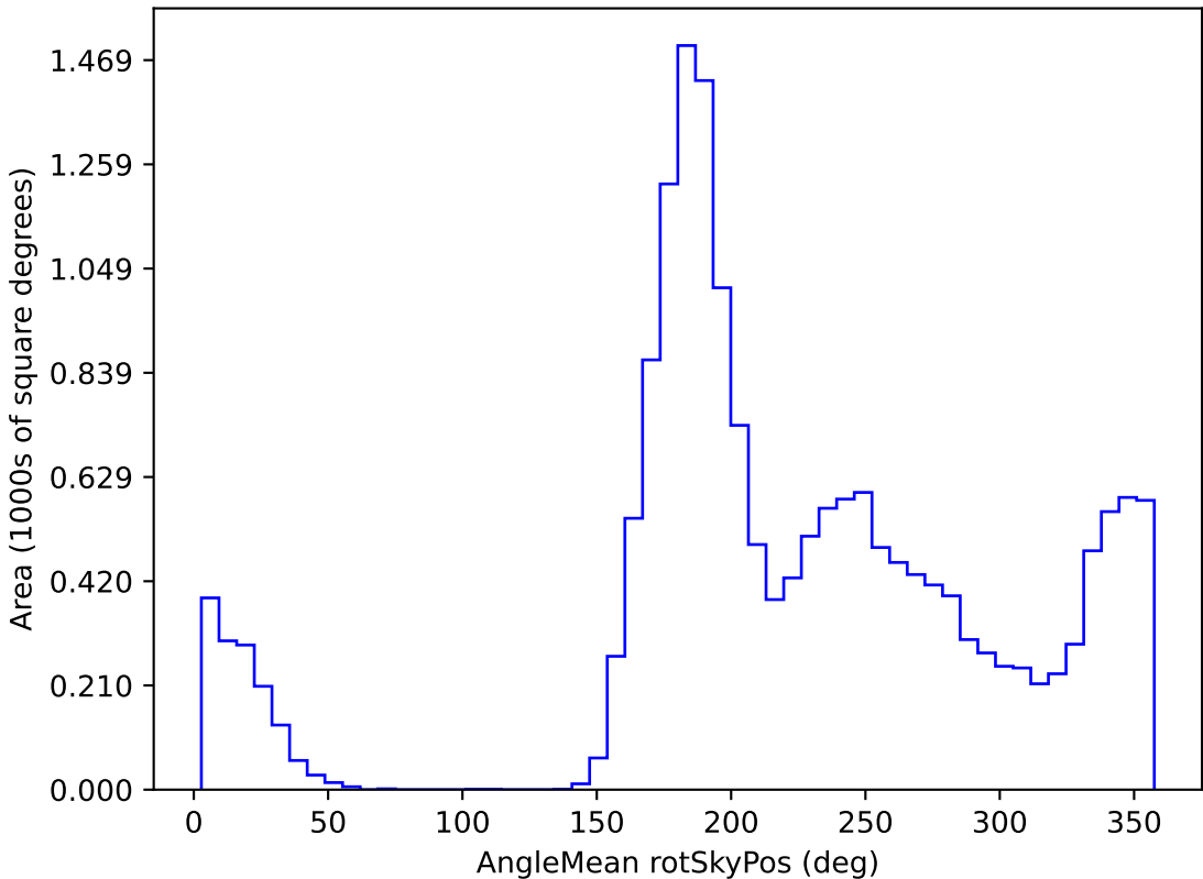
ddf_loaded_fl1_v3.4_10yrs WFD u band: AngleMean rotSkyPos
