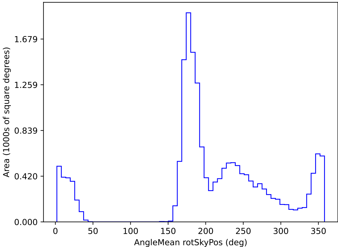
ddf_loaded_fl1_v3.4_10yrs WFD r band: AngleMean rotSkyPos
