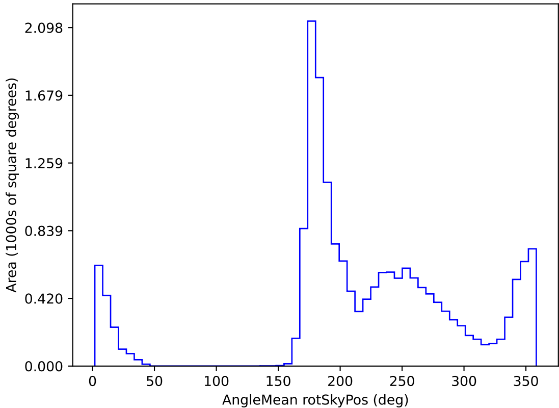
ddf_loaded_fl1_v3.4_10yrs WFD i band: AngleMean rotSkyPos
