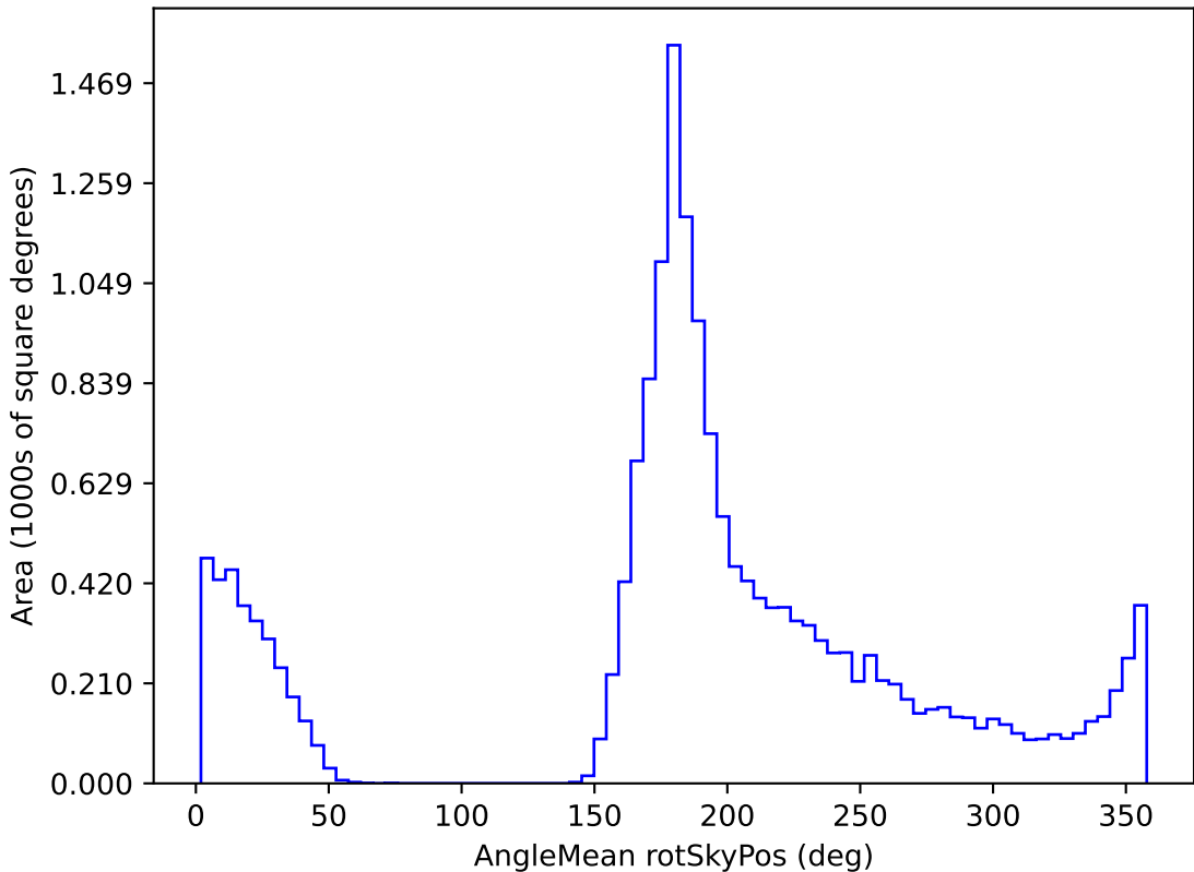
ddf_loaded_fl1_v3.4_10yrs WFD g band: AngleMean rotSkyPos
