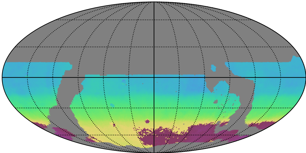
ddf_loaded_fl1_v3.4_10yrs WFD all bands: AngleMean rotSkyPos
