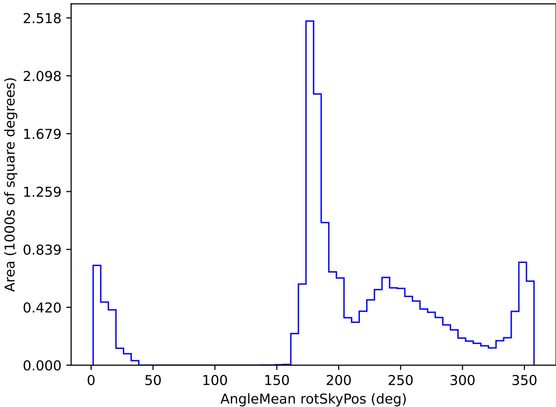
ddf_loaded_fl1_v3.4_10yrs WFD all bands: AngleMean rotSkyPos
