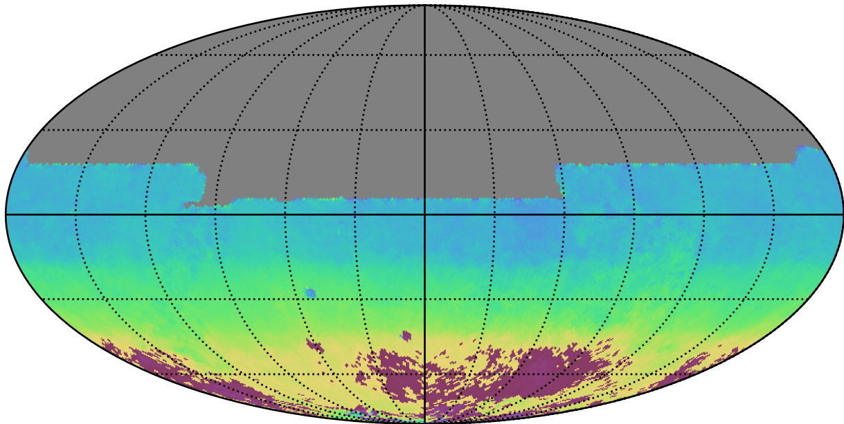
ddf_loaded_fl1_v3.4_10yrs All sky y band: AngleMean rotSkyPos
