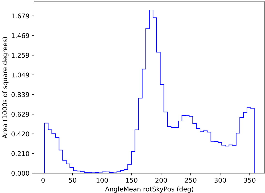
ddf_loaded_fl1_v3.4_10yrs All sky u band: AngleMean rotSkyPos
