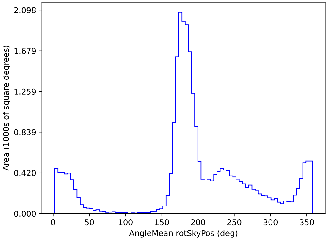
ddf_loaded_fl1_v3.4_10yrs All sky r band: AngleMean rotSkyPos
