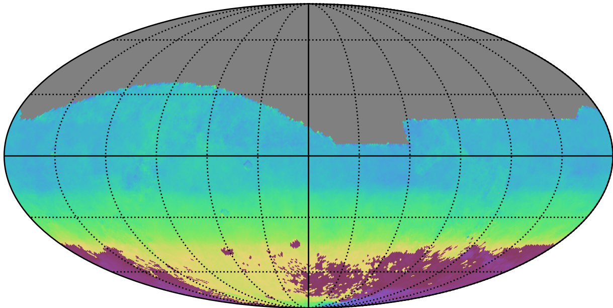
ddf_loaded_fl1_v3.4_10yrs All sky i band: AngleMean rotSkyPos
