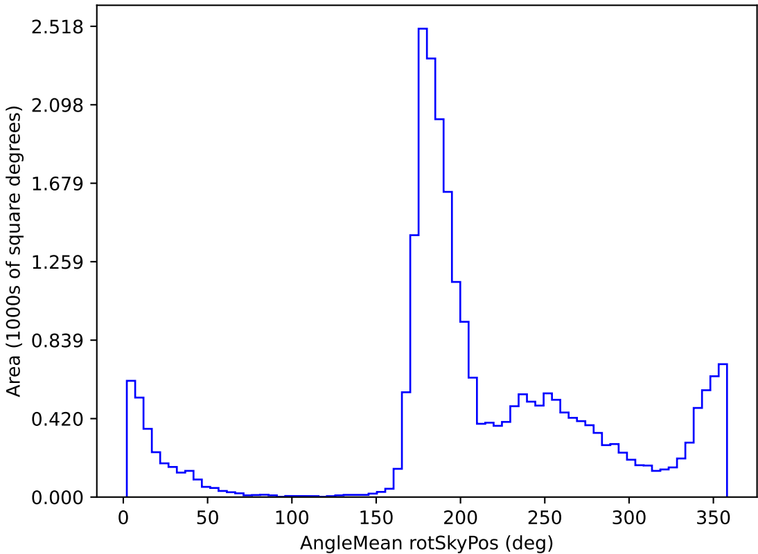
ddf_loaded_fl1_v3.4_10yrs All sky i band: AngleMean rotSkyPos
