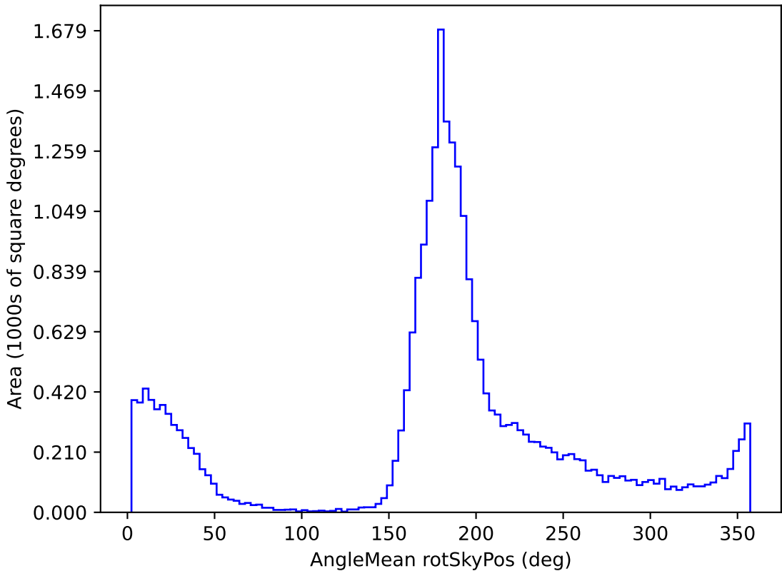
ddf_loaded_fl1_v3.4_10yrs All sky g band: AngleMean rotSkyPos
