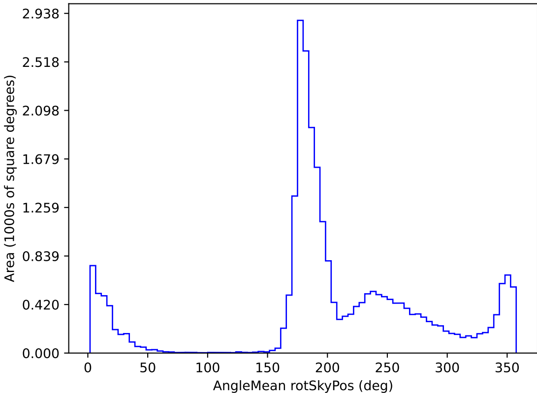
ddf_loaded_fl1_v3.4_10yrs All sky all bands: AngleMean rotSkyPos
