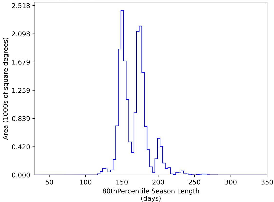
ddf_loaded_fl1_v3.4_10yrs WFD y band: 80thPercentile Season Length
