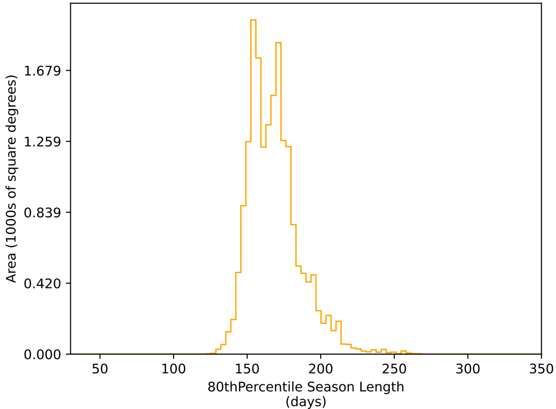
ddf_loaded_fl1_v3.4_10yrs WFD r band: 80thPercentile Season Length
