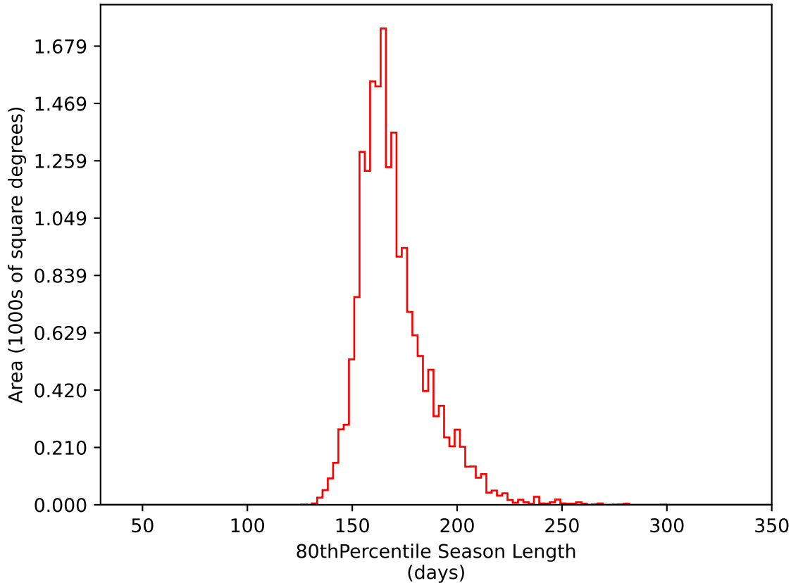
ddf_loaded_fl1_v3.4_10yrs WFD i band: 80thPercentile Season Length
