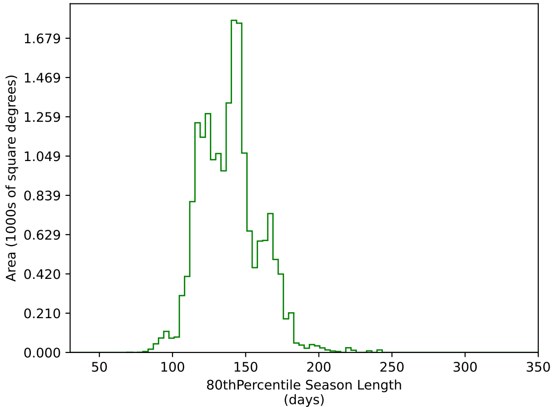
ddf_loaded_fl1_v3.4_10yrs WFD g band: 80thPercentile Season Length
