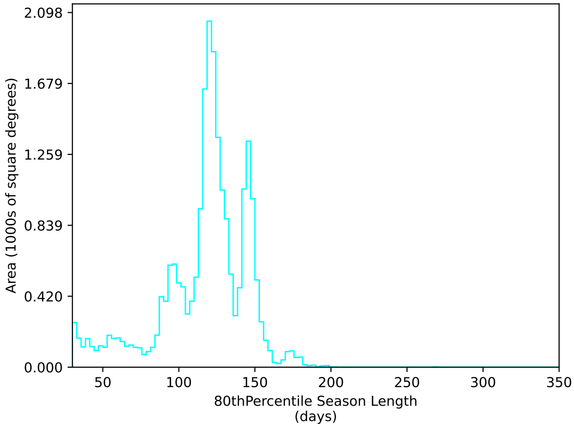
ddf_loaded_fl1_v3.4_10yrs All sky u band: 80thPercentile Season Length
