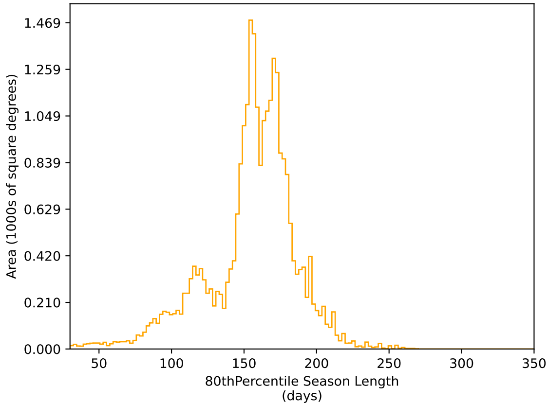
ddf_loaded_fl1_v3.4_10yrs All sky r band: 80thPercentile Season Length
