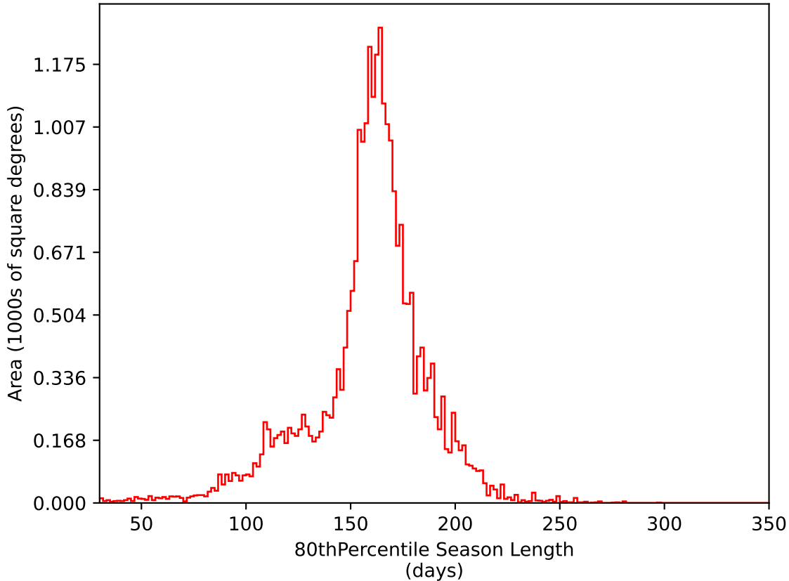
ddf_loaded_fl1_v3.4_10yrs All sky i band: 80thPercentile Season Length
