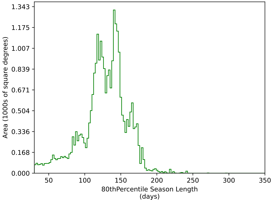
ddf_loaded_fl1_v3.4_10yrs All sky g band: 80thPercentile Season Length
