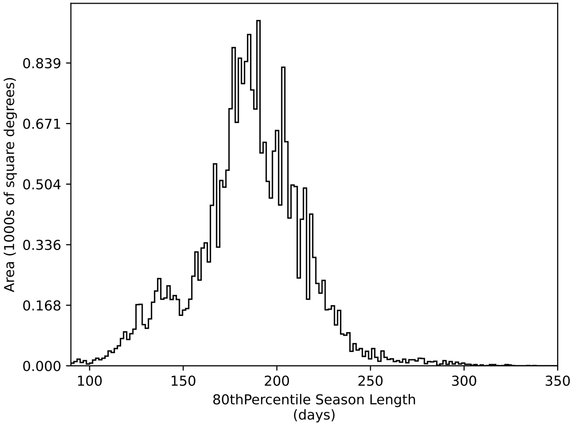
ddf_loaded_fl1_v3.4_10yrs All sky all bands: 80thPercentile Season Length
