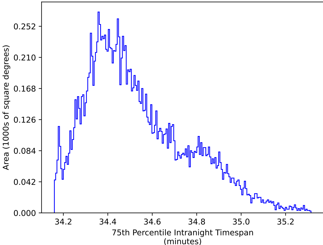
ddf_loaded_fl1_v3.4_10yrs WFD zy bands: 75th Percentile Intranight Timespan
