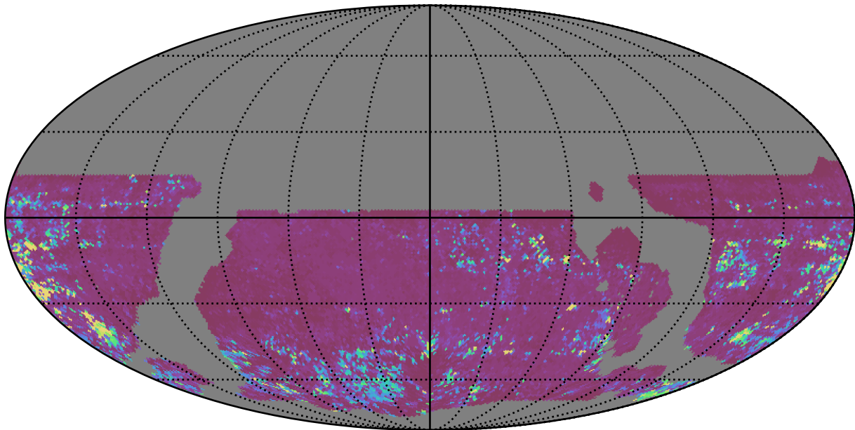
ddf_loaded_fl1_v3.4_10yrs WFD z band: 75th Percentile Intranight Timespan
