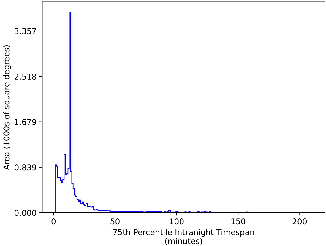
ddf_loaded_fl1_v3.4_10yrs WFD z band: 75th Percentile Intranight Timespan
