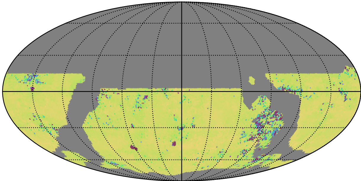
ddf_loaded_fl1_v3.4_10yrs WFD ug bands: 75th Percentile Intranight Timespan
