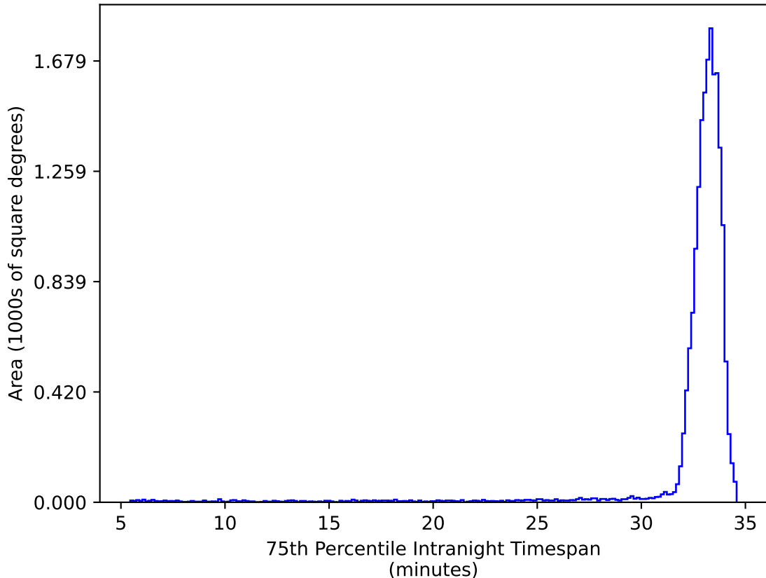
ddf_loaded_fl1_v3.4_10yrs WFD ug bands: 75th Percentile Intranight Timespan
