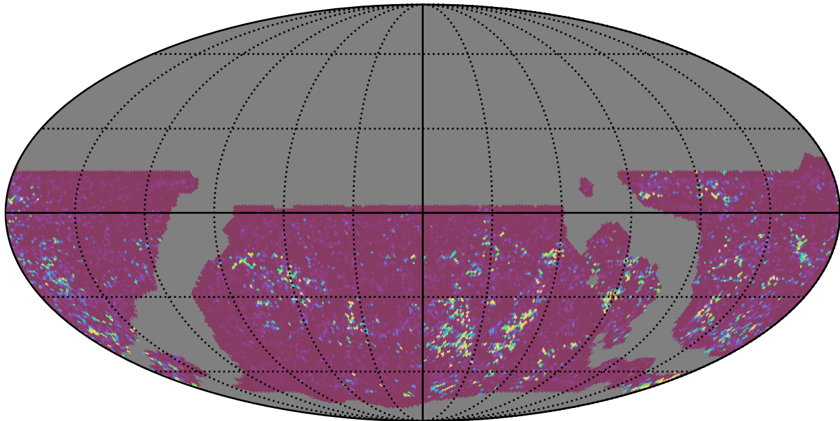
ddf_loaded_fl1_v3.4_10yrs WFD u band: 75th Percentile Intranight Timespan
