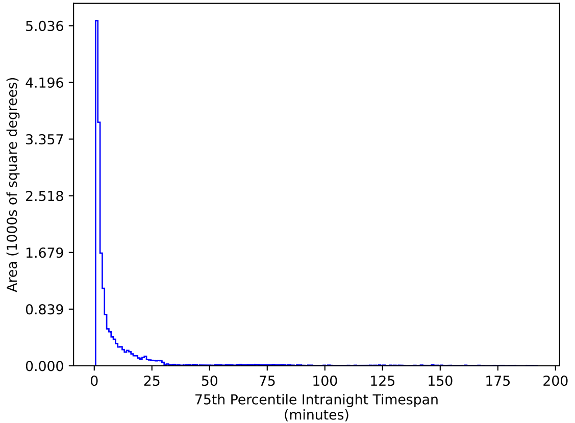
ddf_loaded_fl1_v3.4_10yrs WFD u band: 75th Percentile Intranight Timespan
