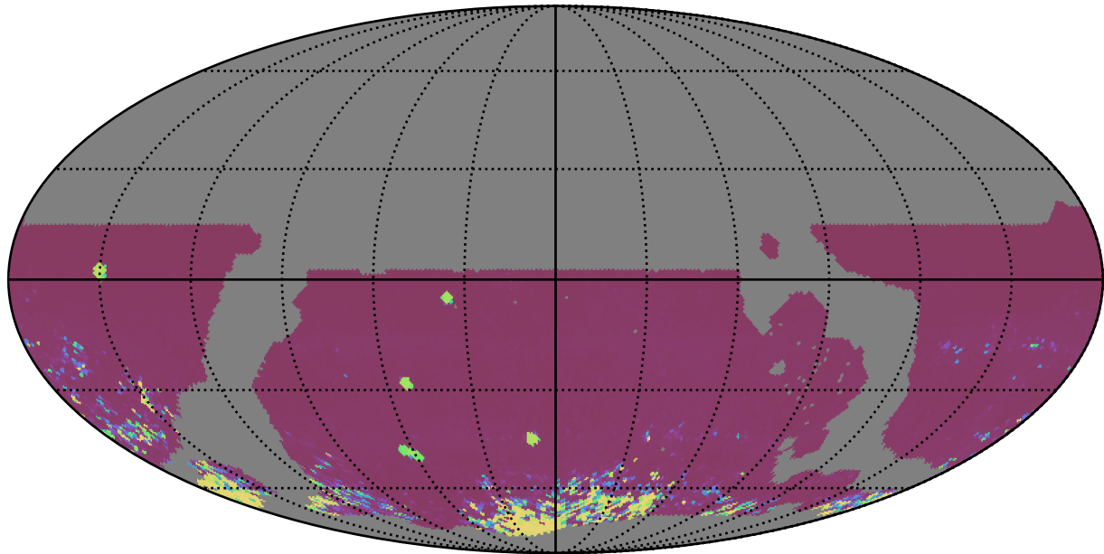
ddf_loaded_fl1_v3.4_10yrs WFD ri bands: 75th Percentile Intranight Timespan
