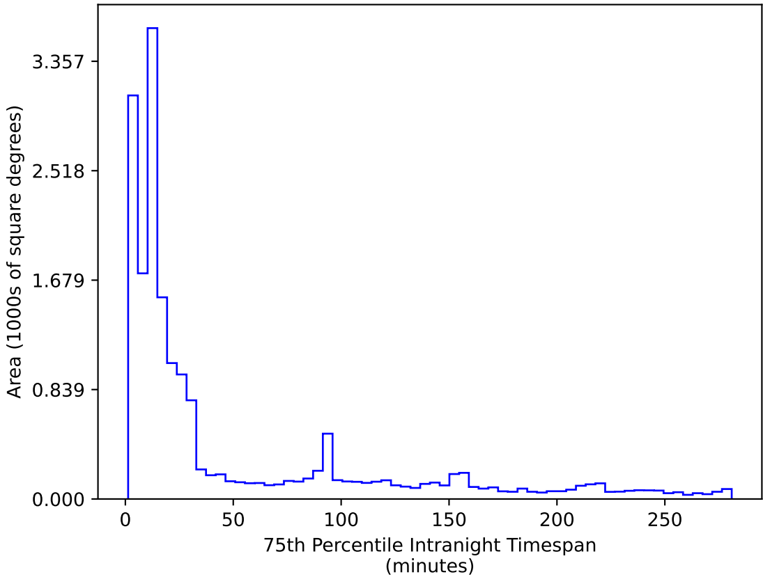
ddf_loaded_fl1_v3.4_10yrs WFD r band: 75th Percentile Intranight Timespan
