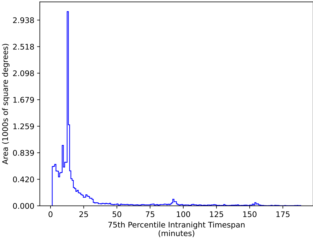
ddf_loaded_fl1_v3.4_10yrs WFD i band: 75th Percentile Intranight Timespan
